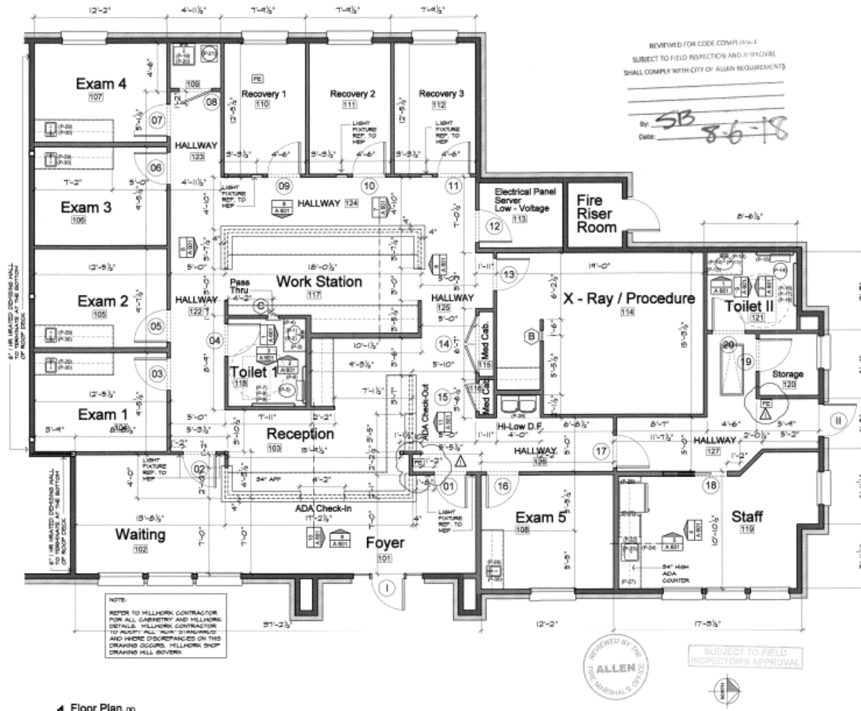
1 Floor Plan (x) SCALE: 1/4" = 1'-0" AREA: 3,198 SQ. FT.
